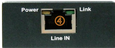
Receiver (RX)-Rear
